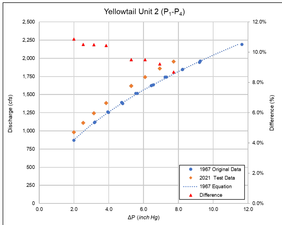
Figure 10.—Comparison of test data from 2021 to the original 1967 test for Yellowtail Powerplant taps P 1 –P 4 .
