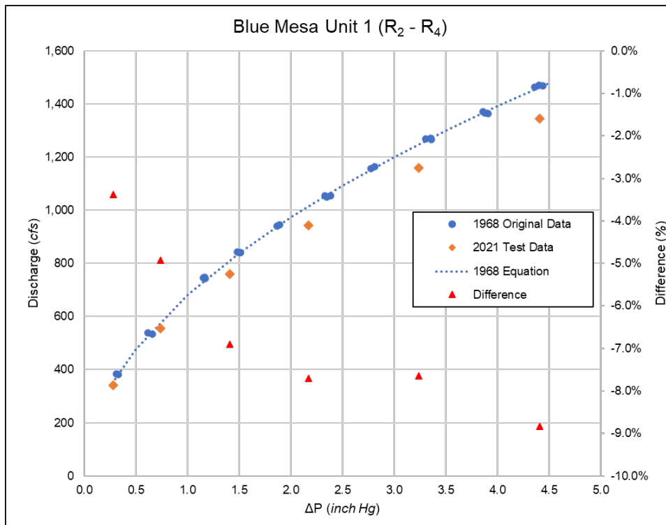
Figure 8.—Comparison of test data from 2021 to the original 1968 test for Blue Mesa Powerplant taps R 2 –R 4 .
