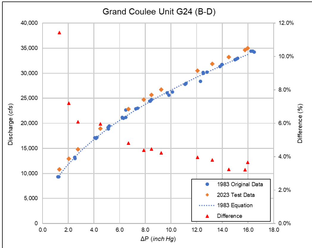
Figure 6.—Comparison of test data from 2023 to the original 1983 test for Grand Coulee Powerplant taps B–D.
