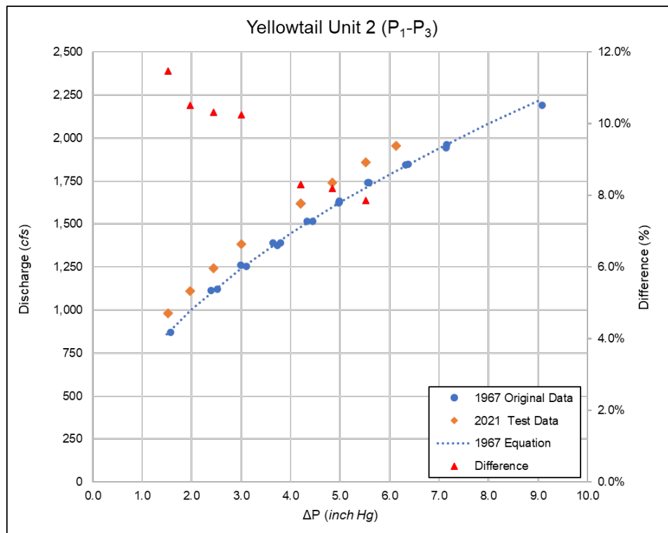
Figure 9.—Comparison of test data from 2021 to the original 1967 test for Yellowtail Powerplant taps P 1 -P 3 .
