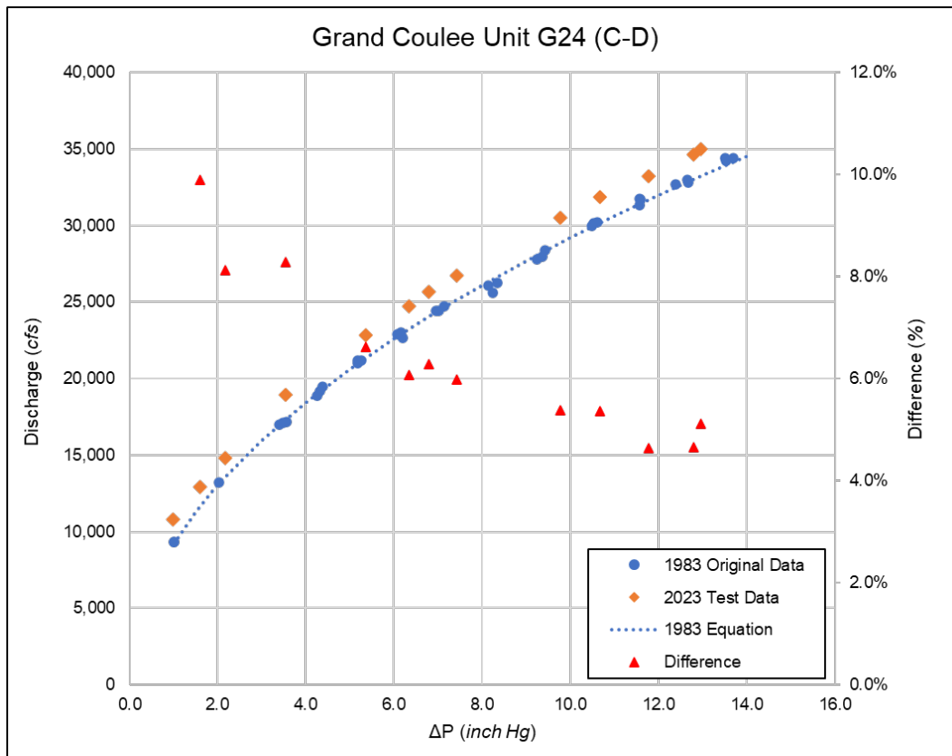
Figure 7.—Comparison of test data from 2023 to the original 1983 test for Grand Coulee Powerplant taps C–D.
