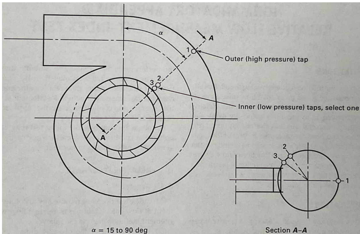
Figure 1.—Schematic of typical Winter-Kennedy pressure taps for a spiral type scroll case, common for Reclamation Francis type turbine runners (ASME 2018).
