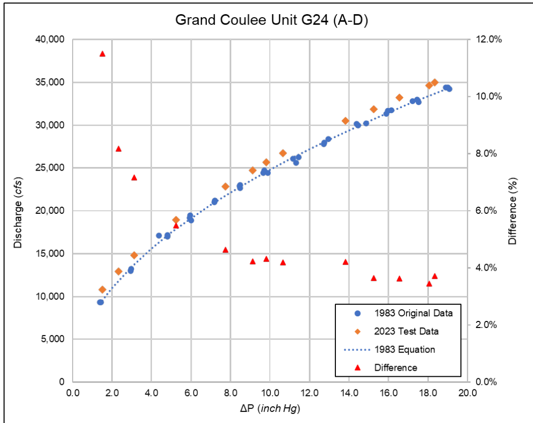
Figure 5.—Comparison of test data from 2023 to the original 1983 test for Grand Coulee Powerplant taps A–D.
